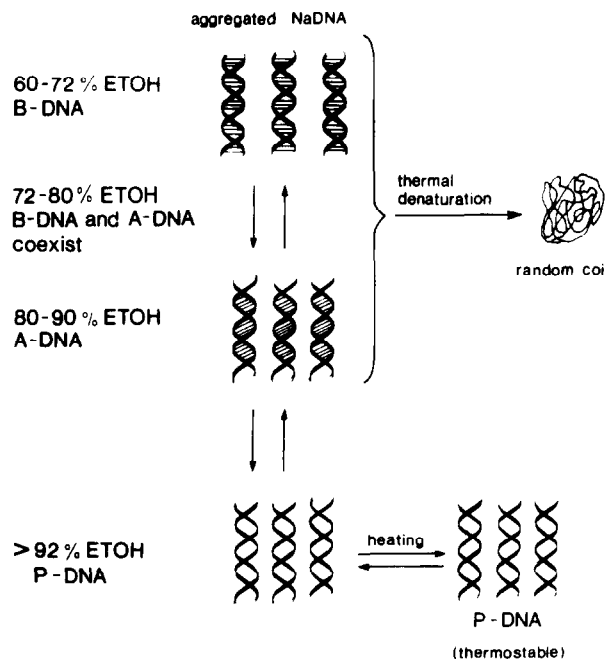
Fig. 4. A simple model describing thermal behaviour of aggregated NaDNA for various ethanol concentrations. Upon thermal denaturation of B-DNA and A-DNA the helix-to-coil transition takes place. In the B-to-A transition region, 72–80% ethanol (EtOH), B-DNA and A-DNA coexist. When transferred to >92% ethanol, NaDNA adopts the P form [37] which has altered secondary structure. Because of the very strong aggregation, P-DNA cannot undergo the helix-to-coil transition and is stable even at very high temperatures.
